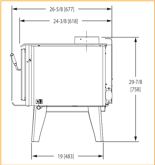
Figure 9.3 - Side View
