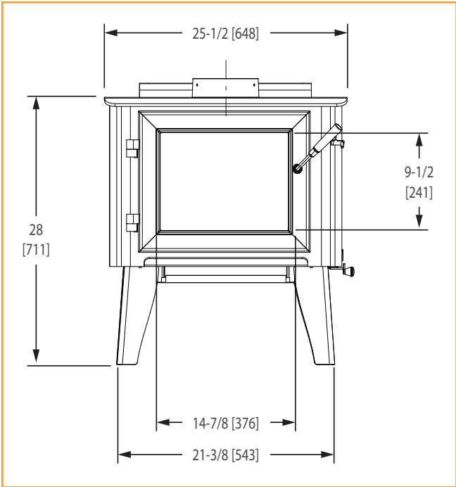
Figure 9.1 - Front View
