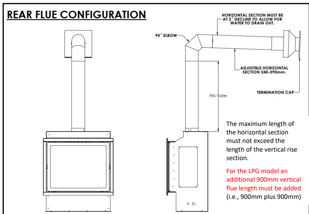
IMAGE 4 - COONARA INBUILT YARRA HORIZONTAL FLUE
